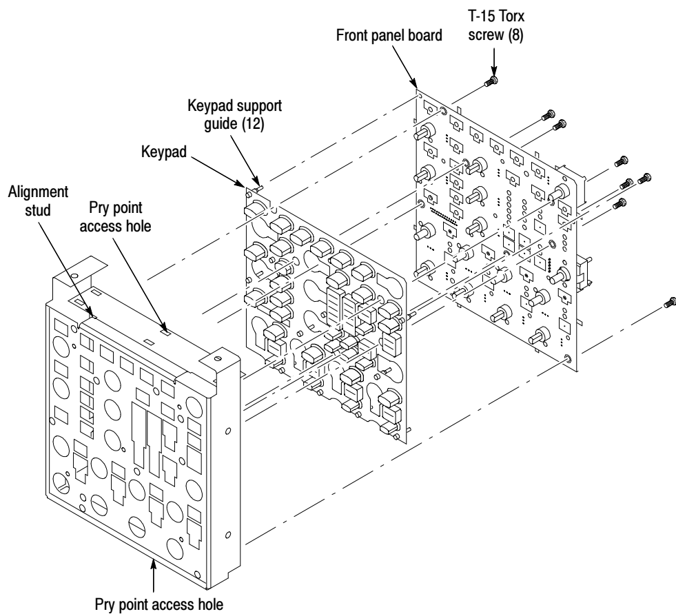
Figure 6-9: Front panel board and keyboard removal
